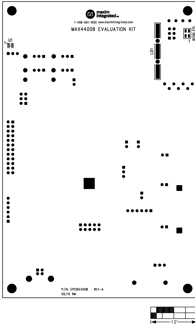
Figure 6. MAX44008 EV Kit Component Placement Guide—Component Side
