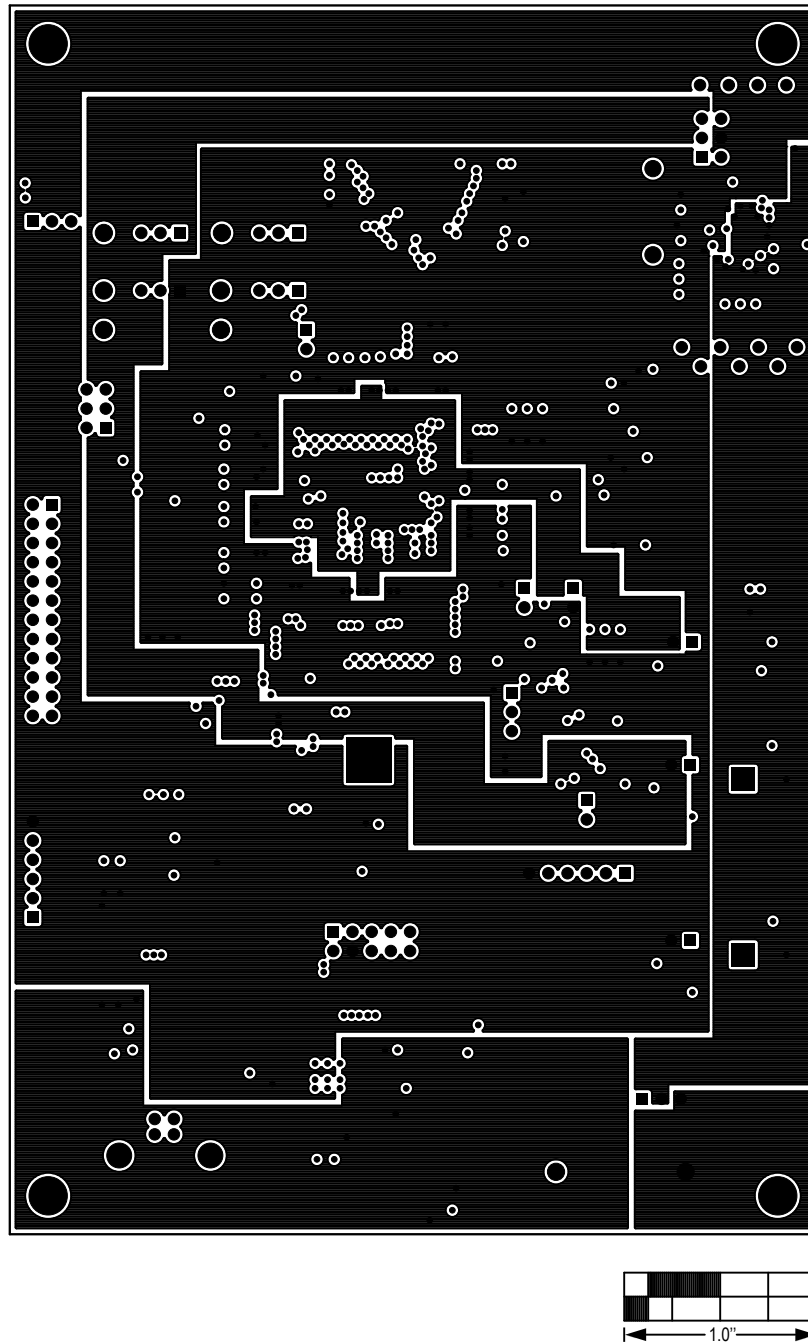
Figure 9. MAX44008 EV Kit PCB Layout—Layer 3
