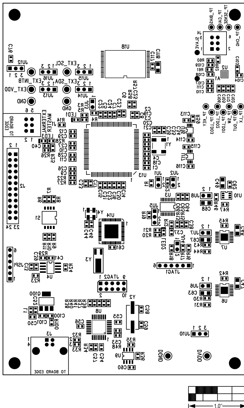
Figure 11. MAX44008 EV Kit Component Placement Guide—Bottom
