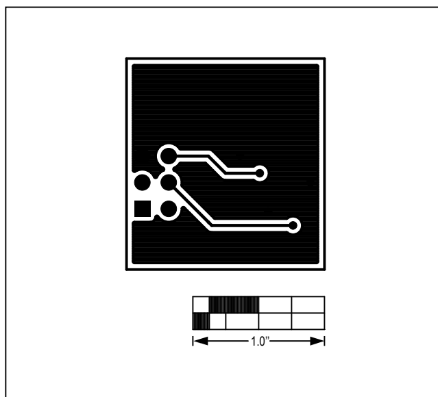
Figure 15. MAX44008 Daughter Board PCB Layout—Bottom
