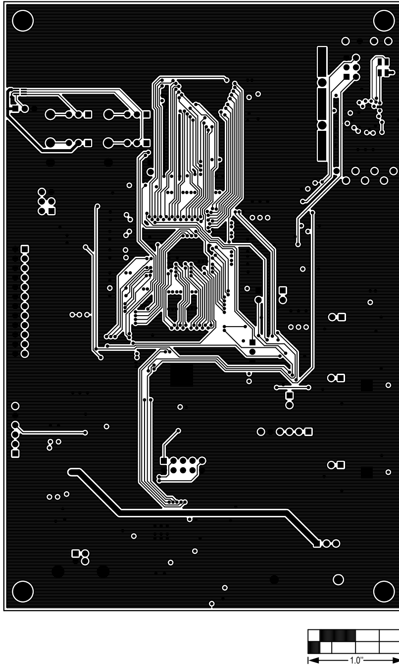
Figure 7. MAX44008 EV Kit PCB Layout—Component Side
