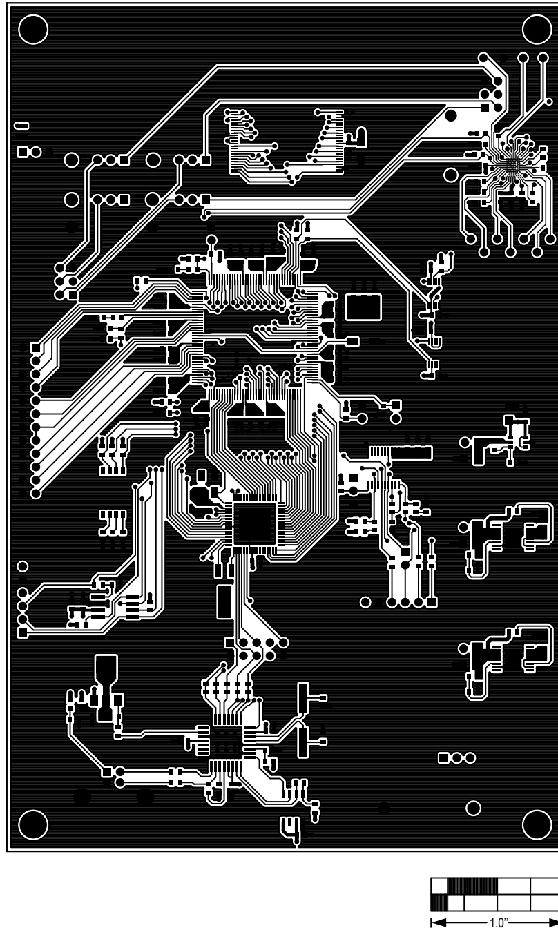
Figure 10. MAX44008 EV Kit PCB Layout—Bottom Side
